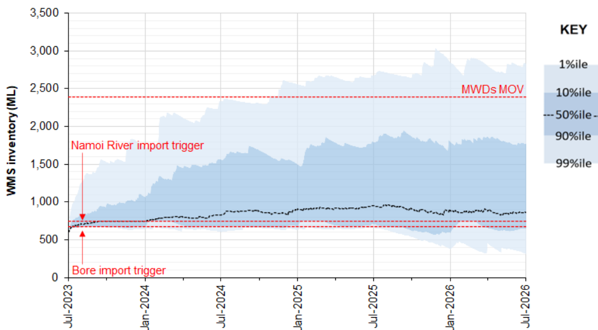
Figure 14 Forecast MWD and Pit Water Storage Combined Inventory
