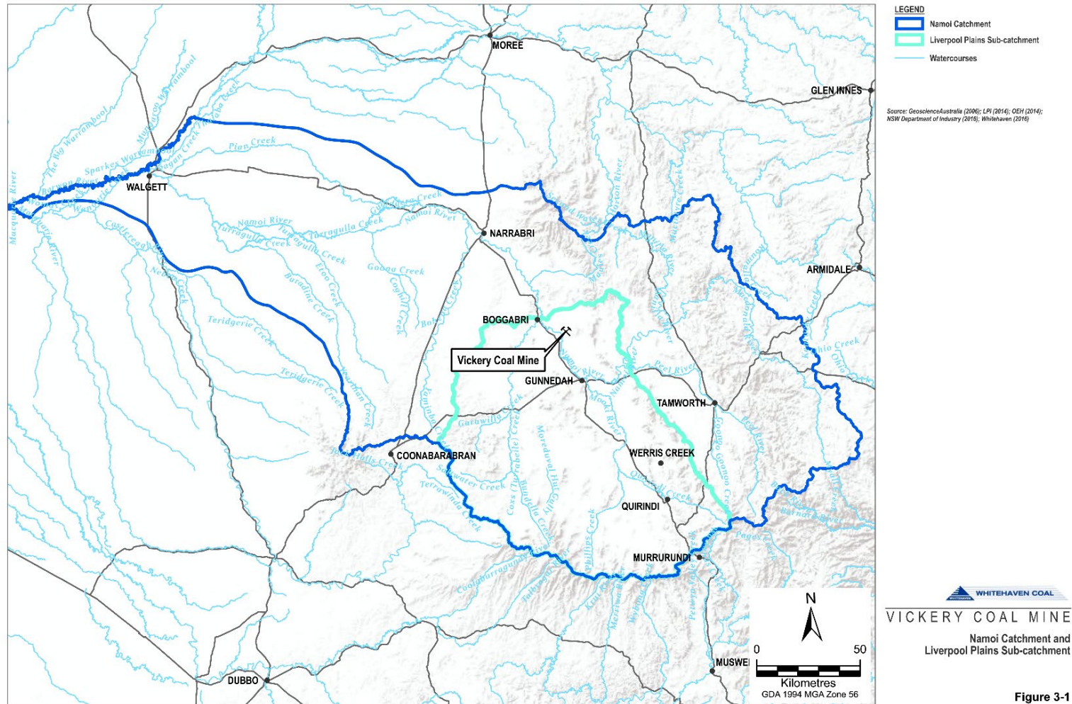
Figure 4 Namoi Catchment and Liverpool Plains Sub-Catchment
