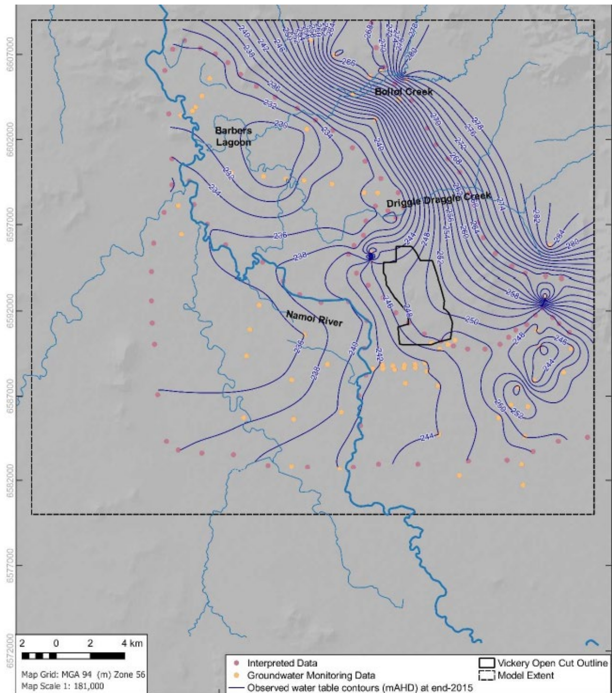
Figure 7-2 Baseline Observed water table (post Canyon and Rocglen mines) (hydrosimulations, 2018)
