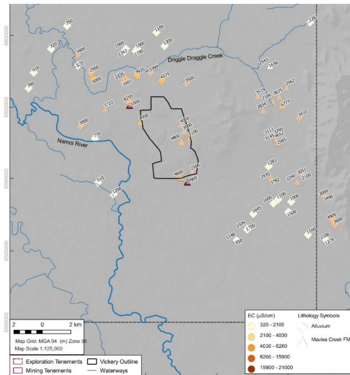
Figure 7-4 Baseline regional water EC from bore census 2012 (Hydrosimulation, 2018)
