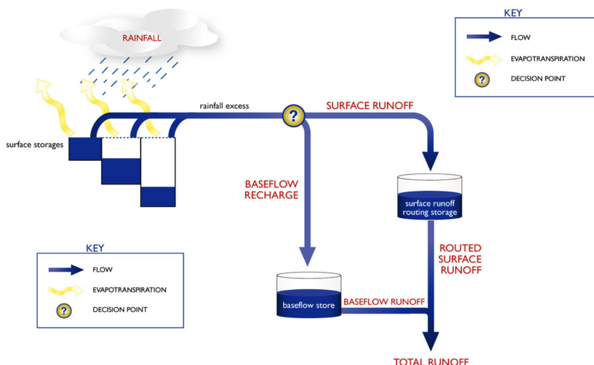
Figure 13 AWBM Model Configuration
