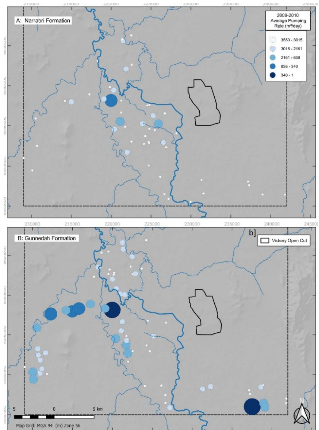
Figure 7-5 Baseline water users in the vicinity of the project (Hydrosimulation, 2018)
