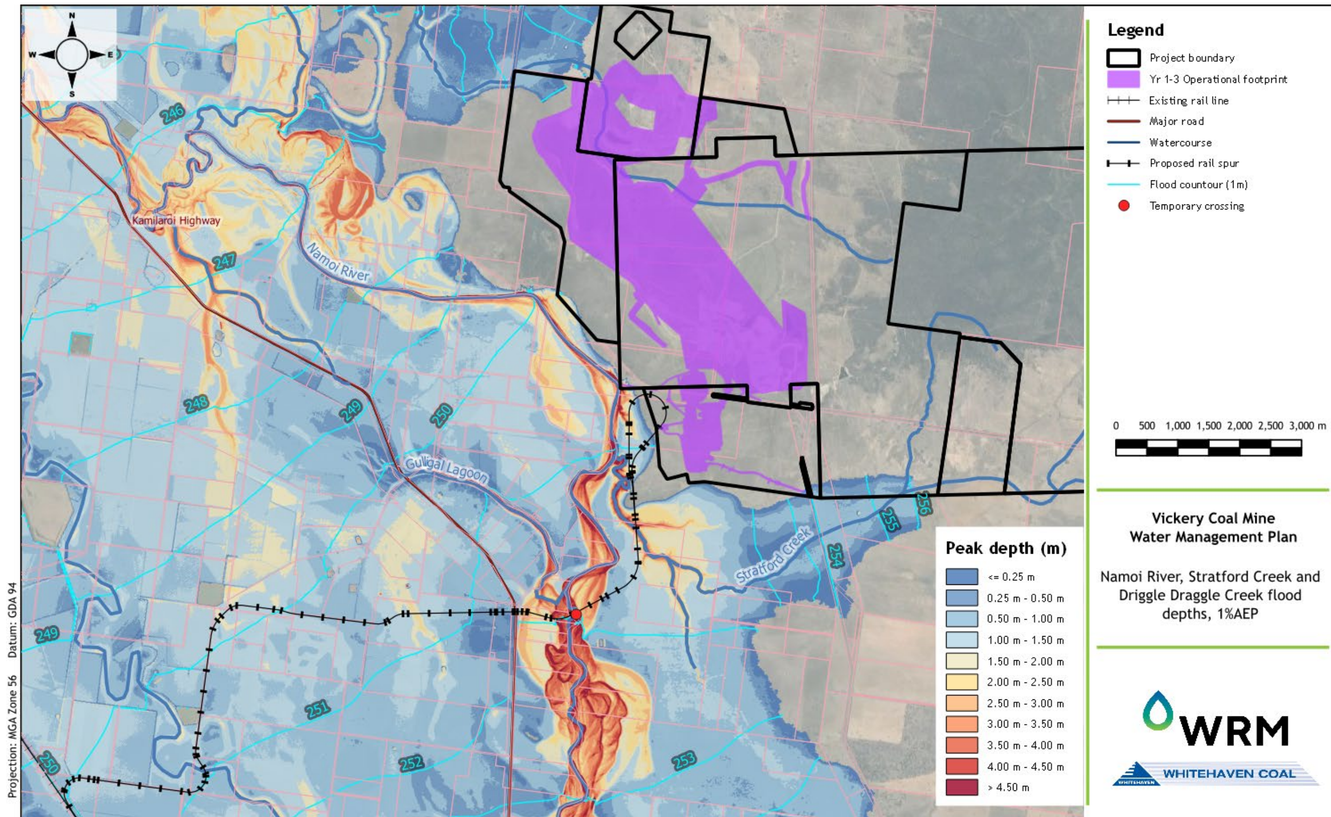
Figure 9 Namoi River Floodplain Depths and Extents for the 1% AEP Event and temporary Namoi River crossing
