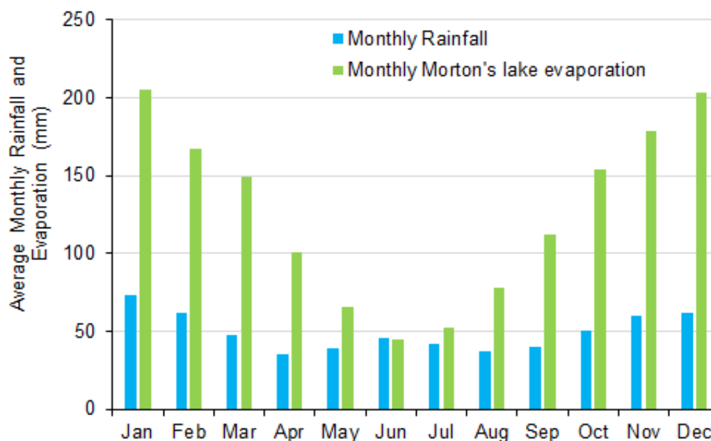
Figure 12 Average Monthly Rainfall and Evaporation from SILO Database
