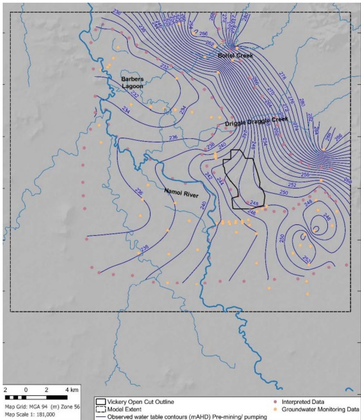
Figure 7-1 Baseline regional water table pre mining (hydrosimulations, 2018)
