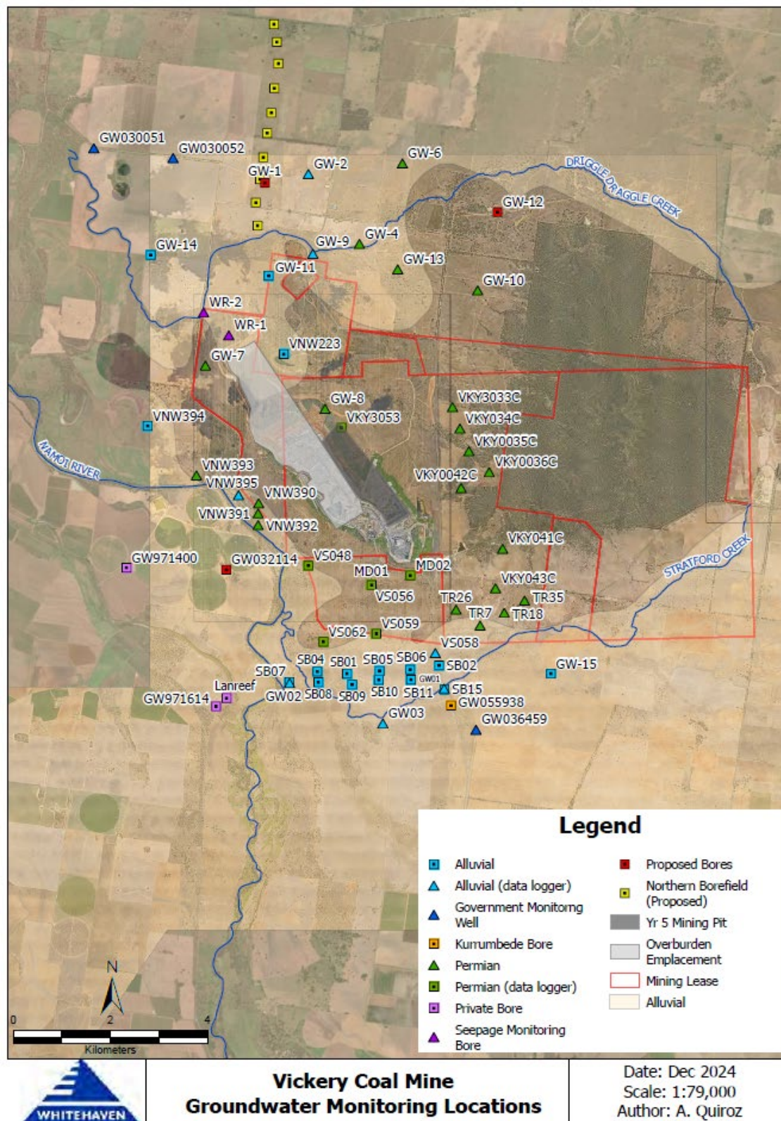
Figure 4-1 VCM Groundwater Monitoring Network
