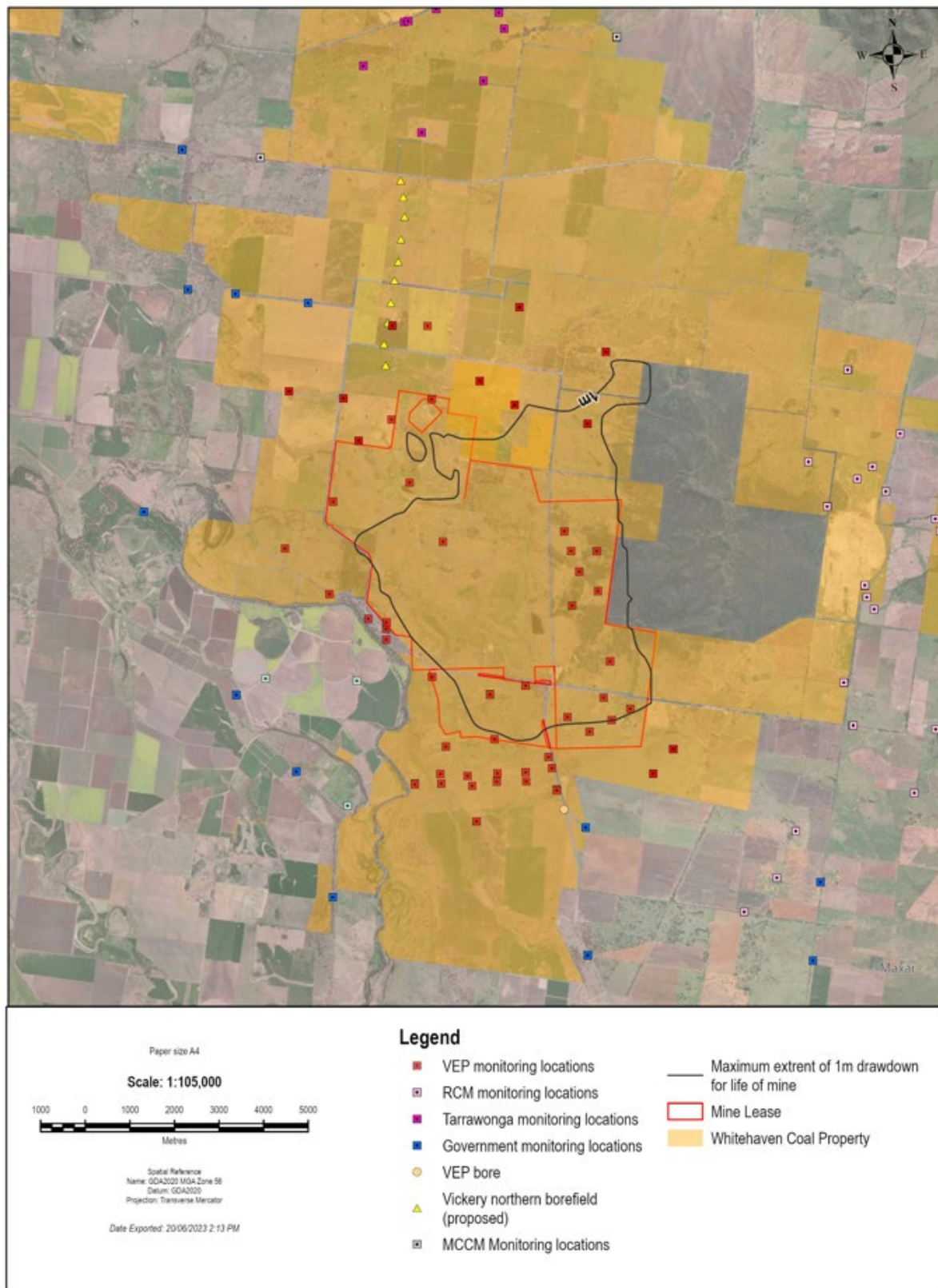
Figure 4-2 Regional Monitoring Network
