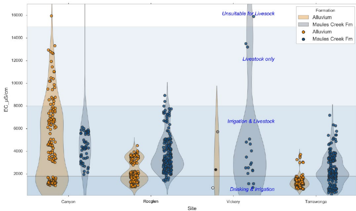
Figure 7-3 Violin Plots showing ranges in EC for Groundwater in the vicinity of Vickery and other Whitehaven mines (Hydrosimulation, 2018)
