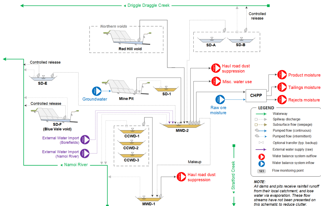
Figure 11 Schematic of Mine Water Management Circuit
