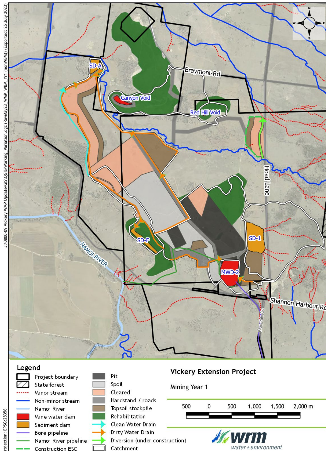
Figure 2a Layout at End of Year 1 (2023)
